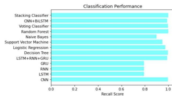
Fig 17: Recall comparison graph
