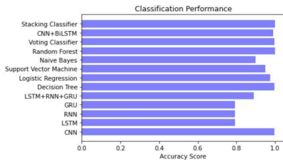
Fig 18: Accuracy graph
