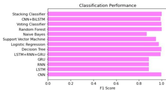
Fig 19: F1Score
