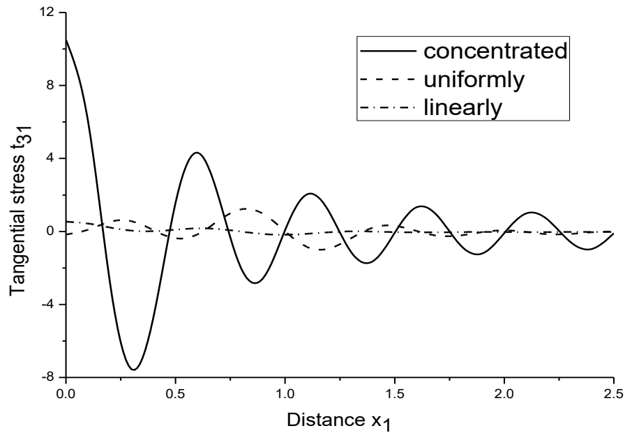
FIGURE 2 BEHAVIOUR AND VARIATION OF t_{31} FOR UNIFORMLY DISTRIBUTED FORCE AND LINEAR DISTRIBUTED SOURCE ARE OPPOSITE TO EACH OTHER FOR 0 < x_1 < 1.98 AND THEN CONVERGES TO EACH OTHER AS x_1 ADVANCES. VALUE OF t_{31} REMAINS HIGHER AS THE POINT OF APPLICATION OF SOURCE AND THEN REMAIN OSCILLATORY AS x_1 ADVANCES.
