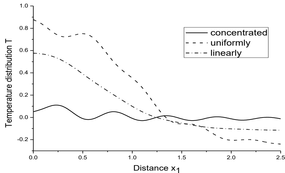
FIGURE 3 MAGNITUDE OF T FOR CONCENTRATED SOURCE AND UNIFORMLY DISTRIBUTION SOURCE REMAINS OSCILLATORY FOR ALL VALUES OF x_1 WHERE AS MAGNITUDE OF T DECREASES MONOTONICALLY AS x_1 INCREASES
