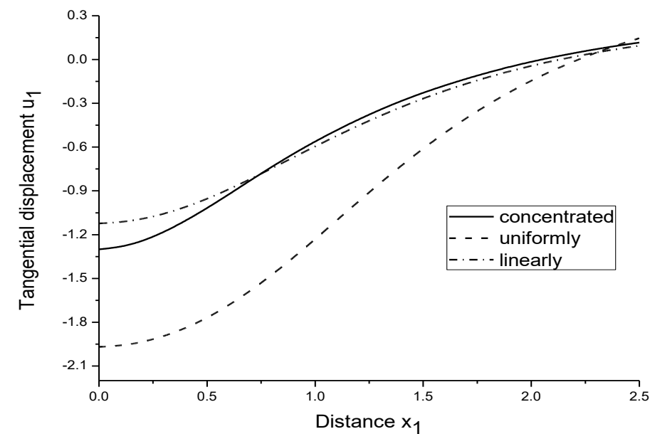
FIGURE 6 THE MAGNITUDES ARE DISTINCT FOR EACH SOURCE APPLIED AS x_1 INCREASES
