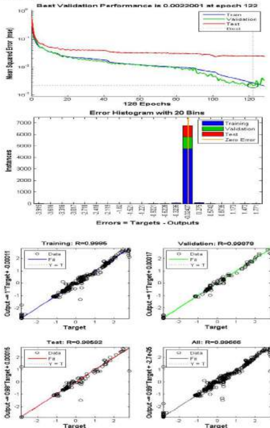
Figure 6: Manner of Regression Analysis
